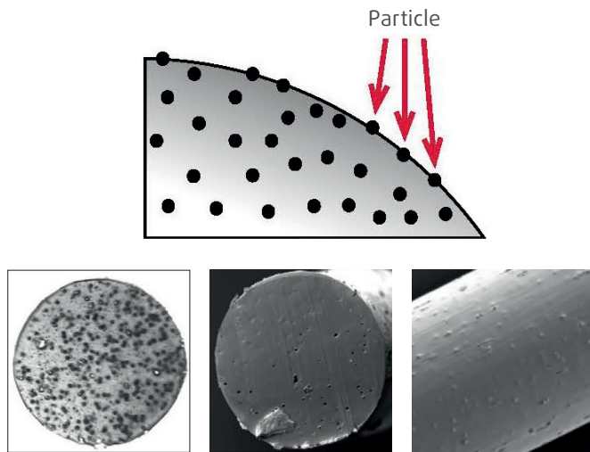
Fig. a - Structure of PearlTech® monofilaments
