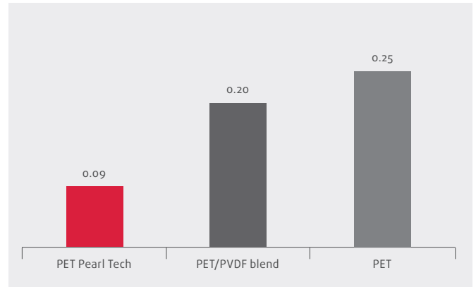
Fig. b - Adhesive force (in N) of polyester-based Adhesives
